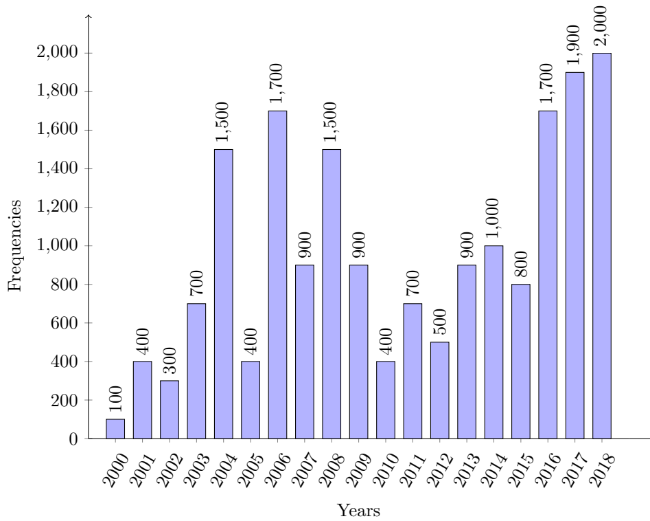
Frequency Histogram
